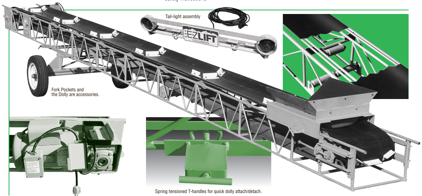
Spring tensioned T-handles for quick dolly attach/detach.
