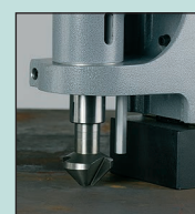
Countersinking
